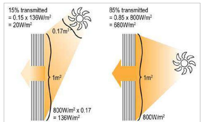
Solar gain varies according to the sun's angle of incidence.
