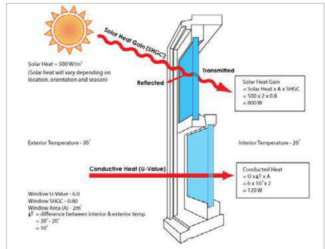
Source: The Australian Window Association Heat transfer mechanisms.
